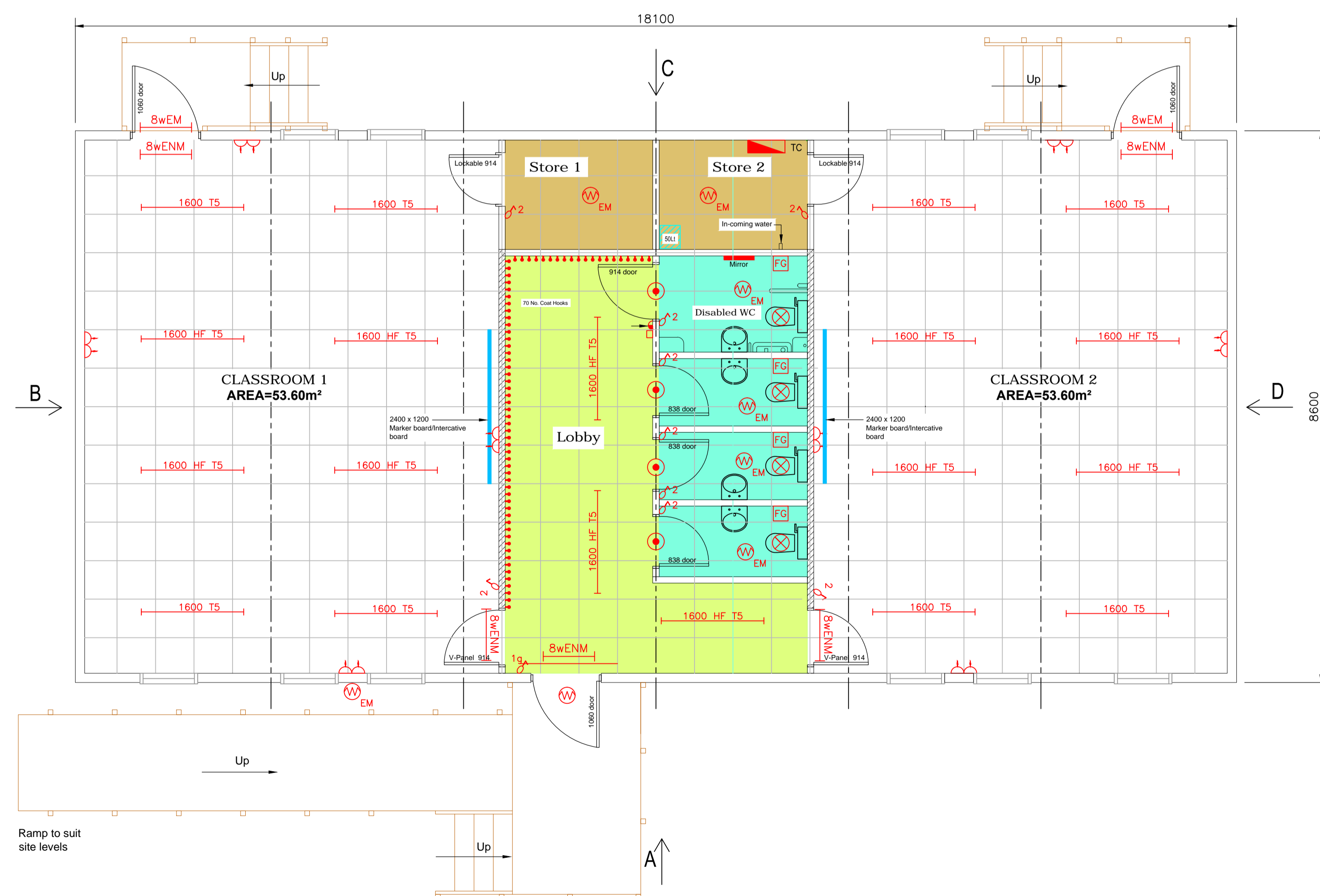
FLOOR PLAN AND ELEVATIONS DRAWING SCALE 1:50
