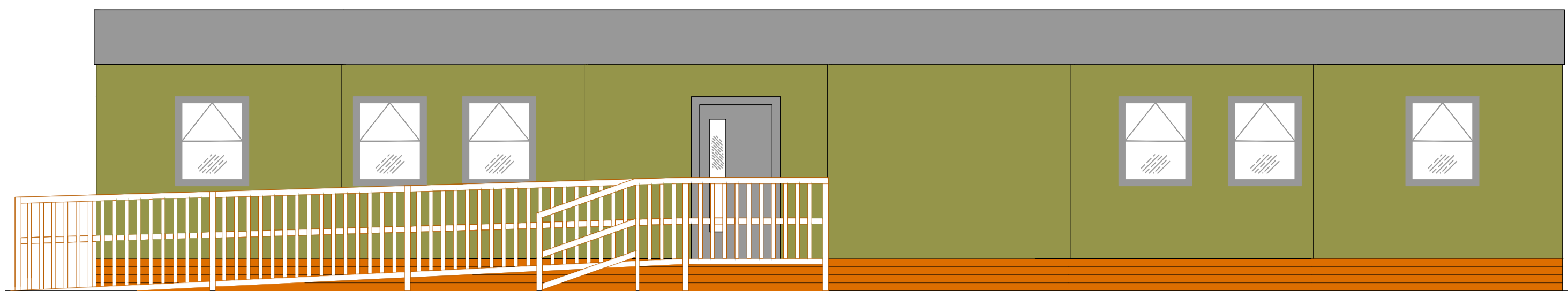
ELEVATION A SCALE 1:50
